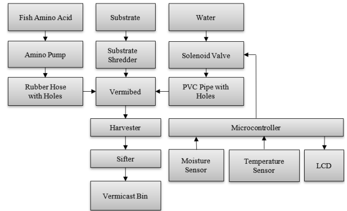
Fig. 1. Block diagram of the device.
