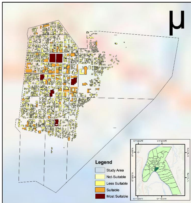
Fig. 7. Solar PV System Installation Suitability Map.
